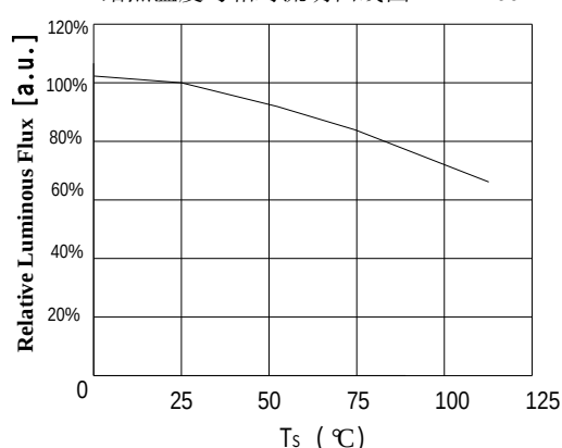
Case Temperature vs. Relative Luminous Flux 结点温度与相对流明曲线图 IF=1100mA
