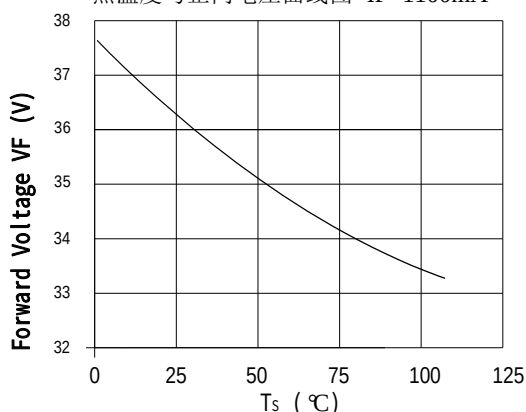
Case Temperature vs. Forward Voltage 结 点温度与正向电压曲线图 IF=1100mA
